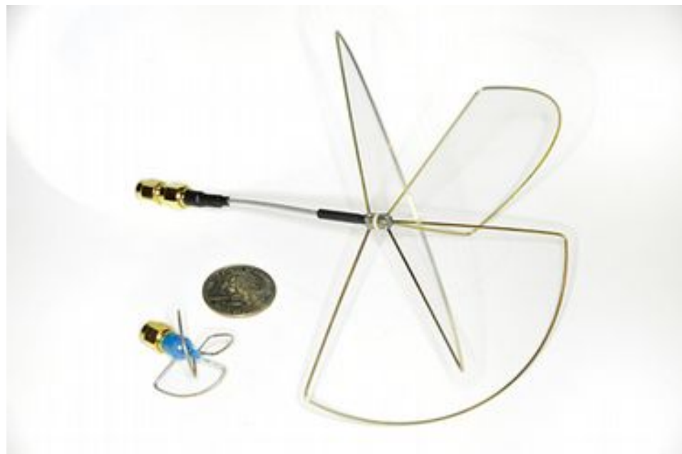
1.3 GHz and 5.8 GHz antenna
